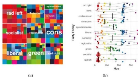
FIGURE 5: Relationship between colour and party family. Cross marks in panel (b) represent colours in national flags.
